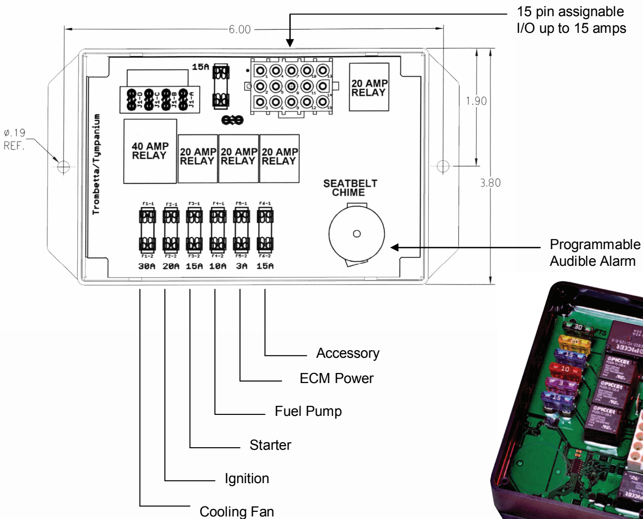
Example of module (electrical diagram example and dimensions of std. box)
