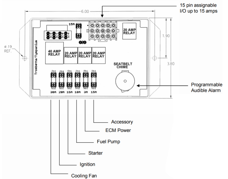
Example of module (electrical diagram example and dimensions of std. box)
